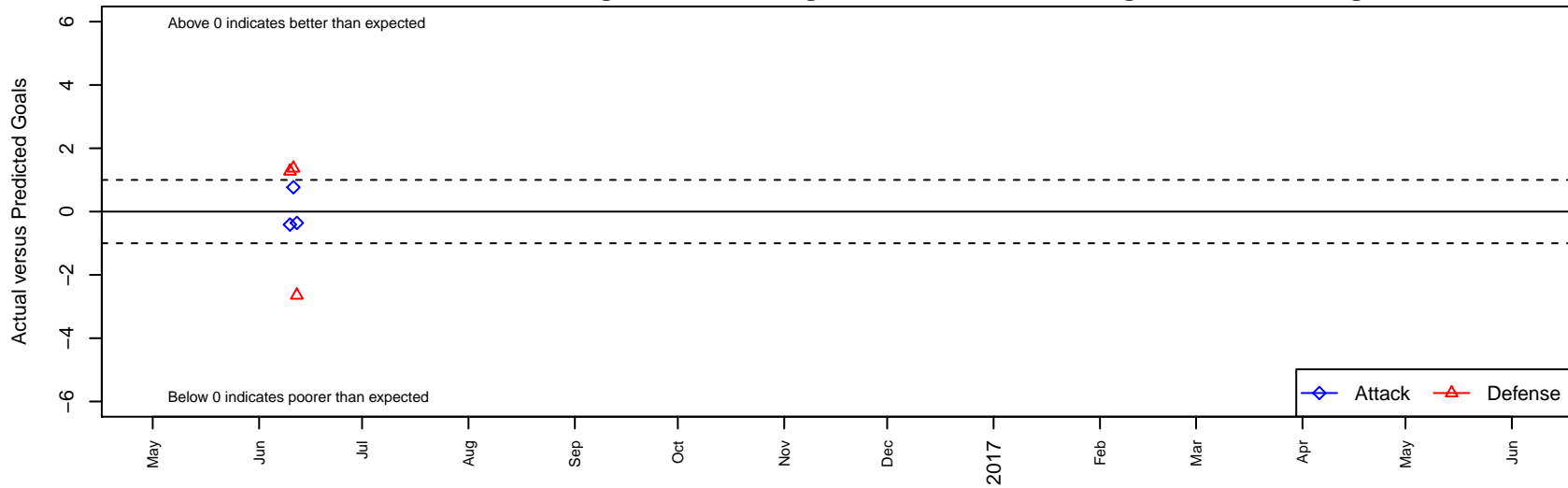
STU Evolution Lopez B04 Dots are actual minus expected GF (blue circles) and GA (red triangles). Blue line is smoothed change in attack strength. Red is smoothed change in defense strength.
